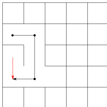
Figure 352: How the recursive backtracker algorithm works (2)
